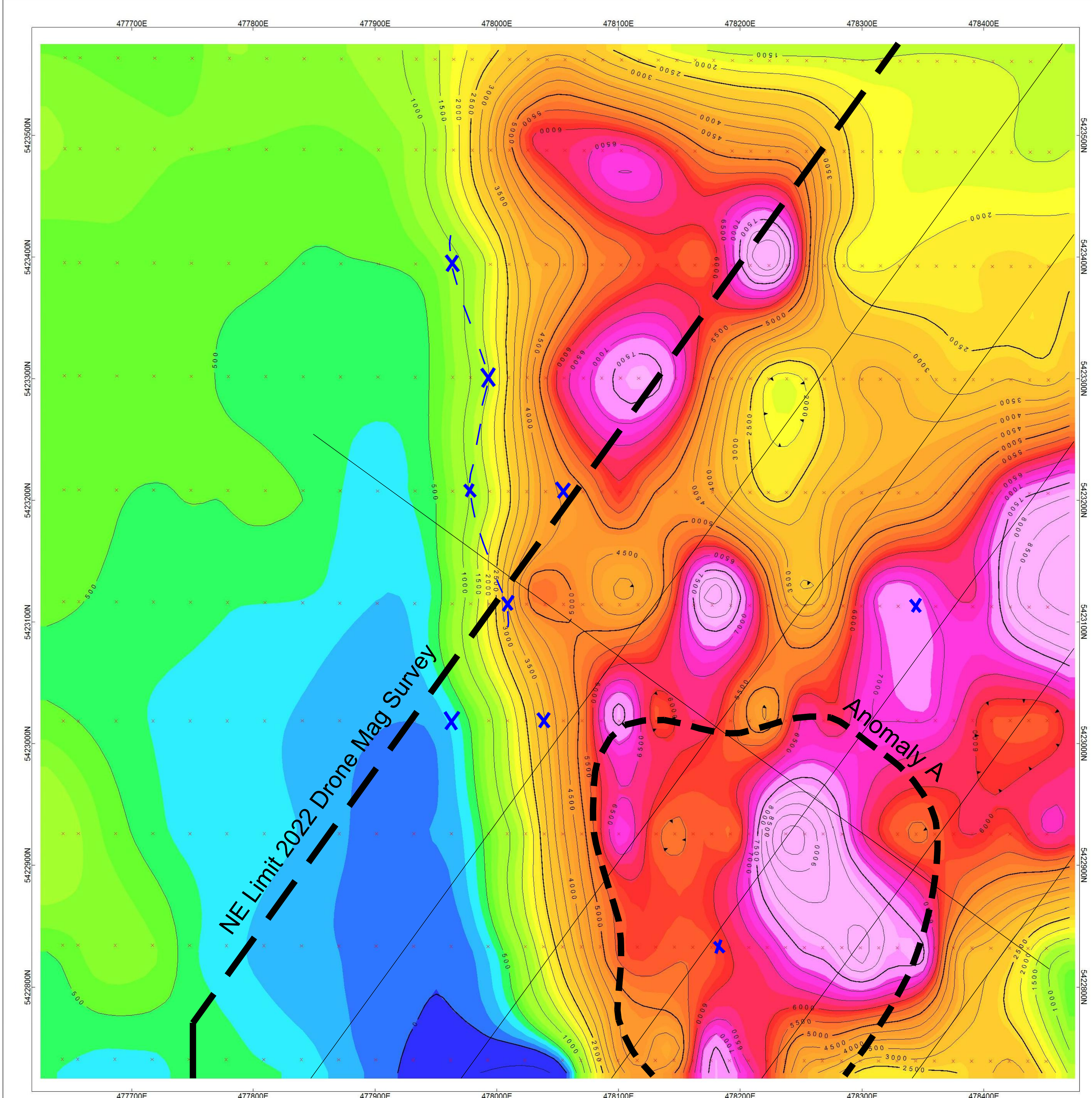
Interpretive Map 2 1964 ground magnetic survey with 2022 Anomaly A outline
